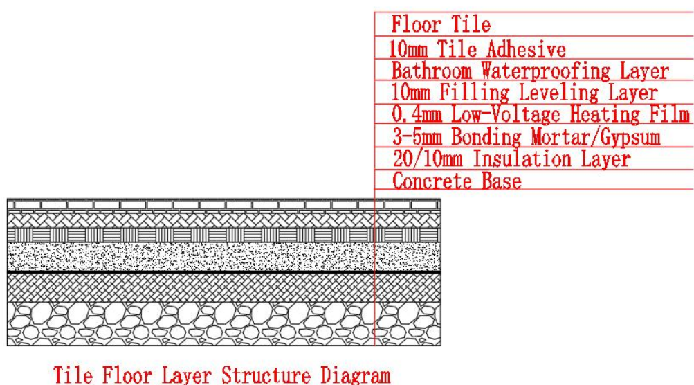
Figure 9.2e — Ceramic tile floor layer diagram
