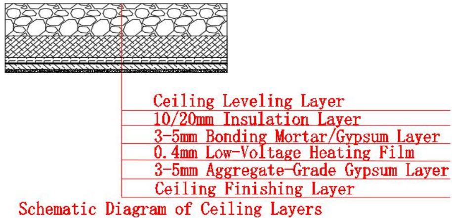
Figure 9.2a — Ceiling layer diagram
